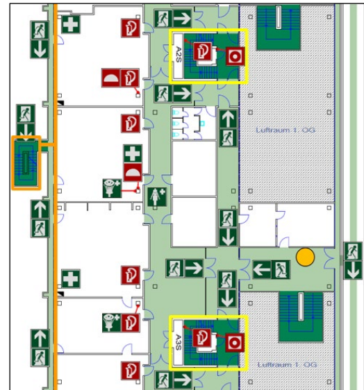
Fig. 1: Example Emergency Escape and Evacuation Plan (Ulmenliet 20, south wing, second)
